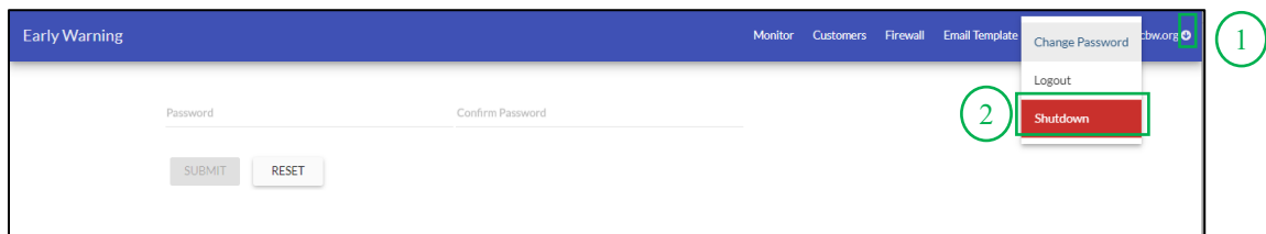
Figure 7 : Shutdown
