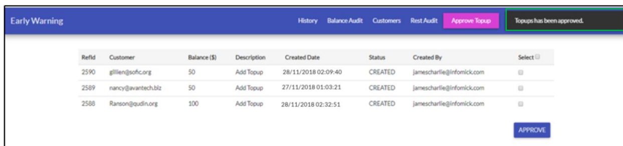
Figure 34: Approved message
