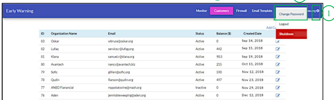
Figure 5 : Changing Password
