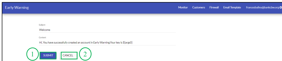
Figure 25 : Submit
