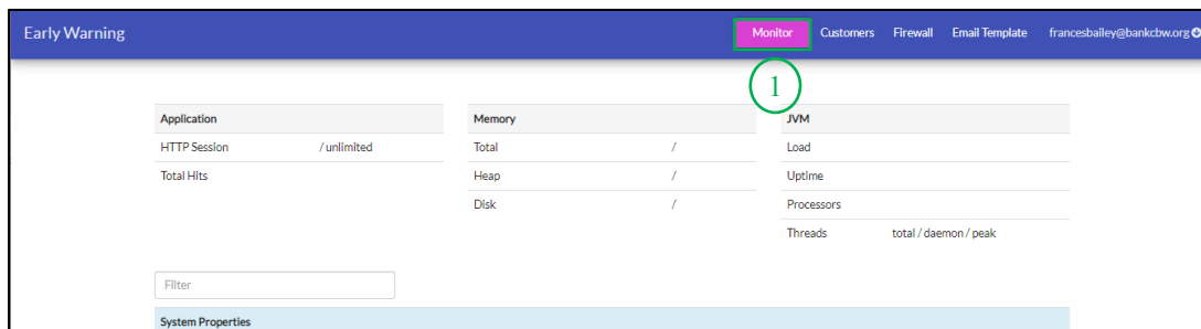
Figure 8 : Monitor
