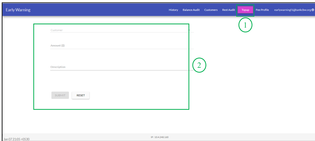
Figure 27: Topup Page
