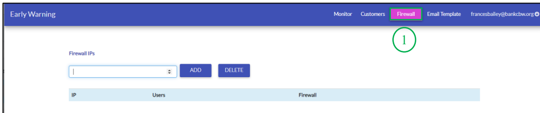
Figure 21 : Firewall page
