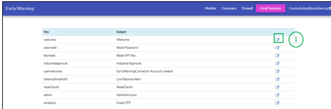
Figure 24 : Edit template
