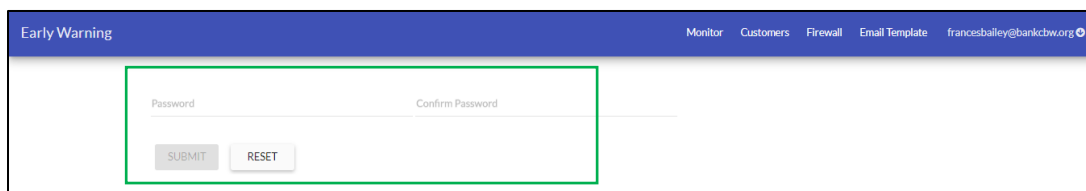
Figure 6 : Changing Password
