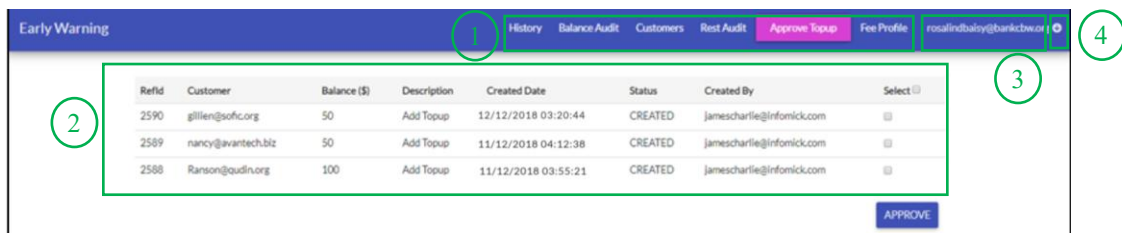
Figure 30: Home Menu
